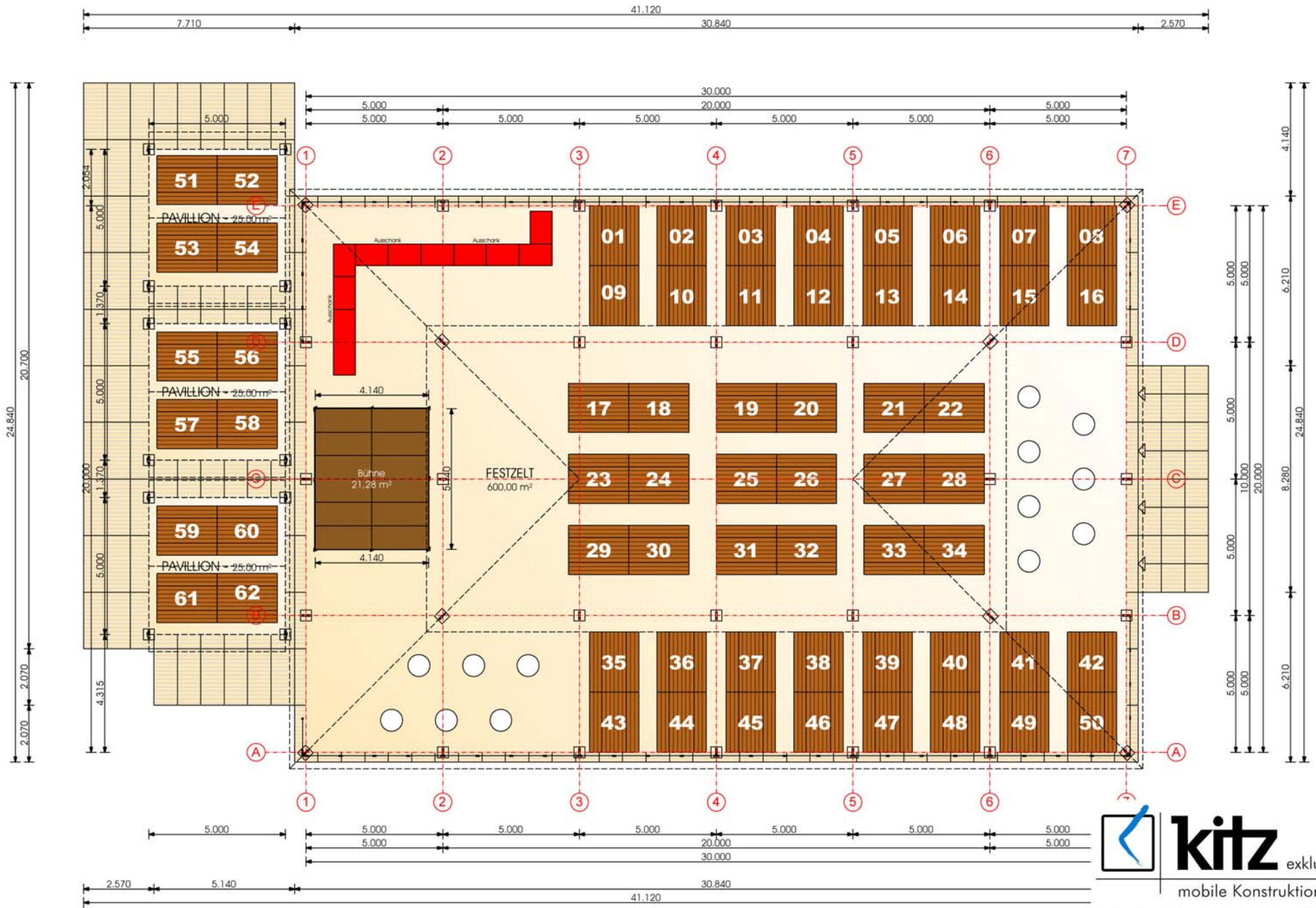
Edelweiss Village (Grundriss)
